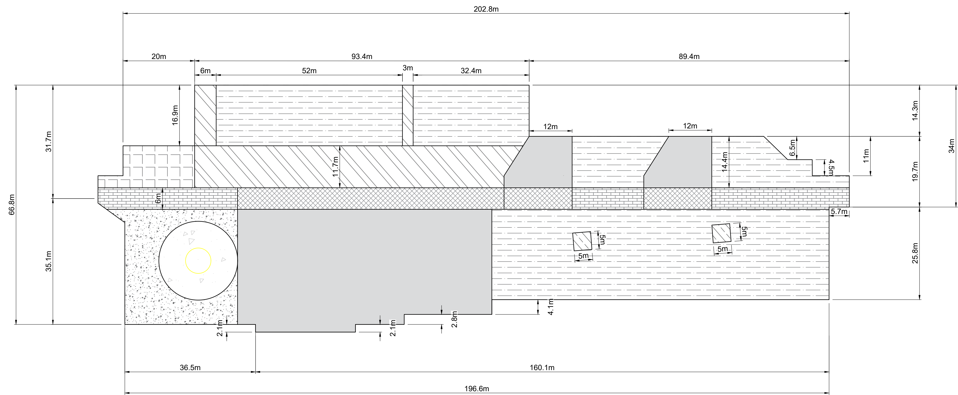
CRANE HARDSTAND - PLAN SCALE 1:500
